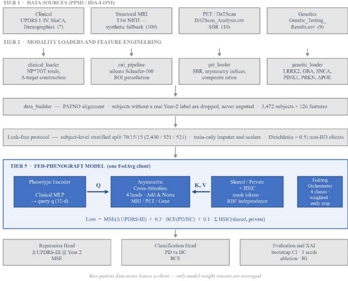
Fig. 2. Fed-PhenoGraft system architecture.
