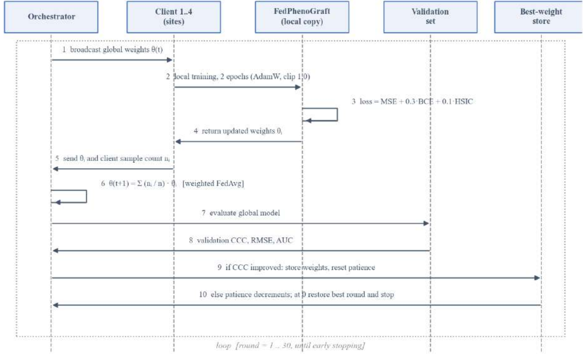
Fig. 7. Sequence diagram - one federated averaging round.
